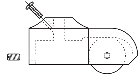
Single Sheave Truck Detail Stationary truck Cast aluminum body Nylon sheave
